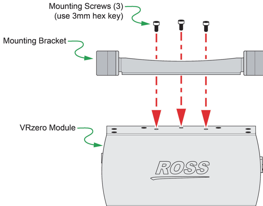
Figure 3.3 - Attaching the Mounting Bracket to the VRzero Module
