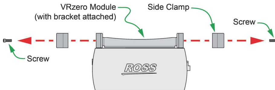
Figure 3.4 - Removing Side Clamps
