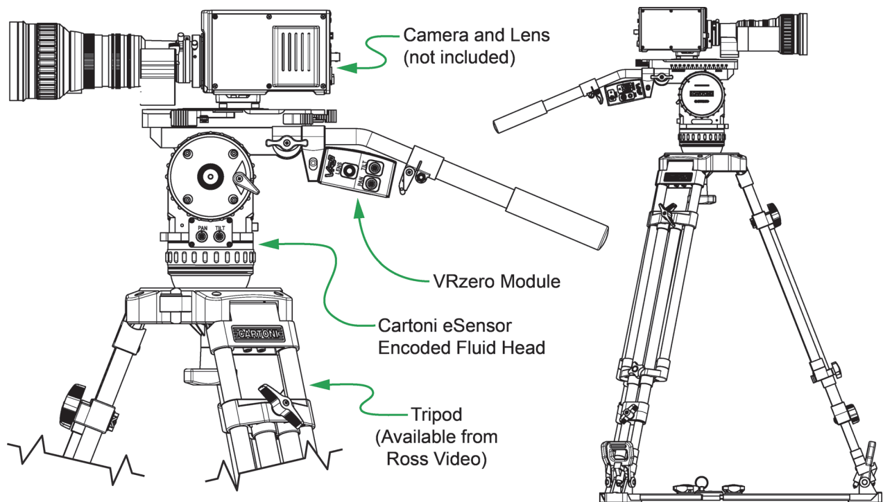
Figure 2.1 - The VRzero eSensor Bundle (cables omitted for clarity)
