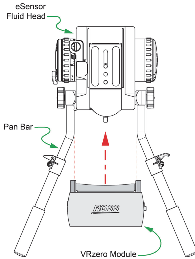
Figure 3.5 - Sliding the VRzero Module onto the Pan Bars
