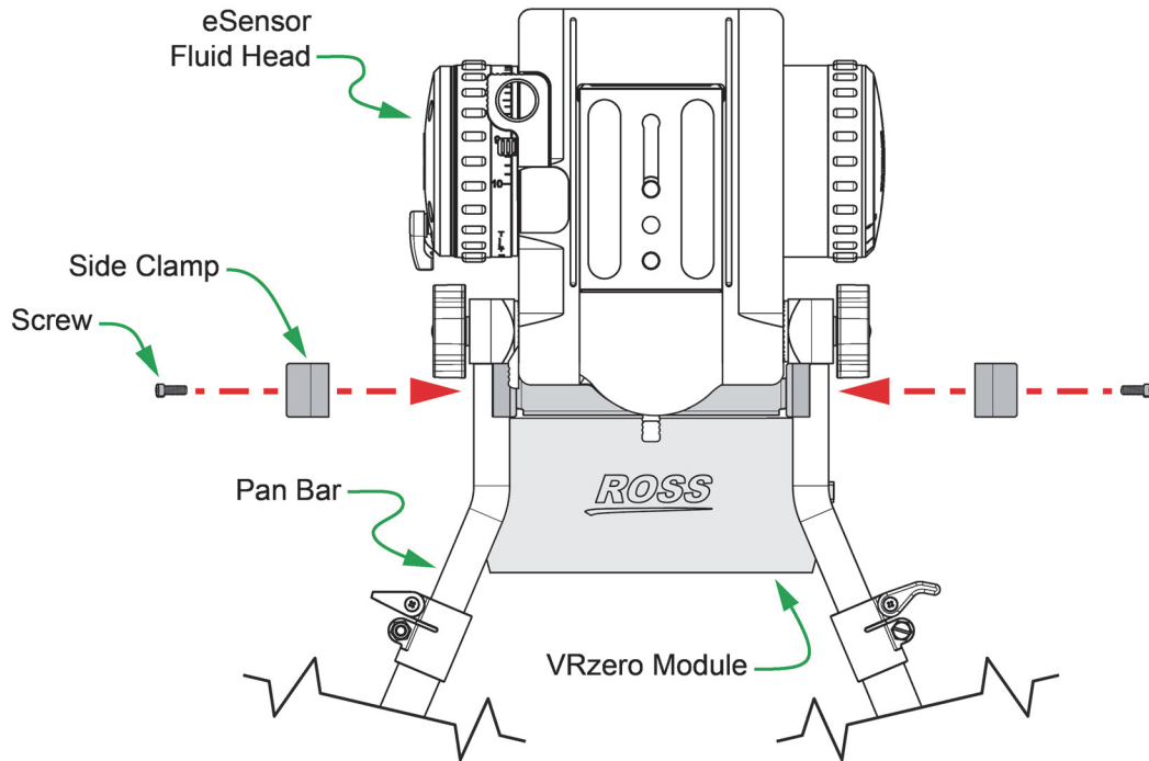
Figure 3.6 - Reattaching the Side Clamps
